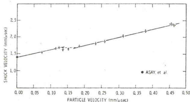
FIG. 5. Measured shock velocity-vs-particle velocity for Teflon. The point at zero particle is from the ultrasonic measurements of Asay et al. (Ref. 14).
