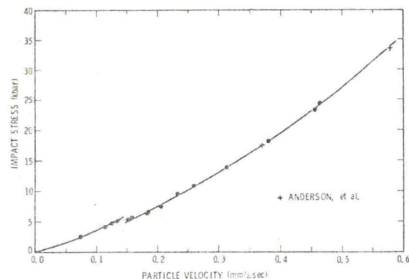
FIG. 4. Shock stress-vs-particle velocity for Teflon as determined from impact-surface measurements. The phase transition is indicated by the change in slope beginning at 5 kbar.
